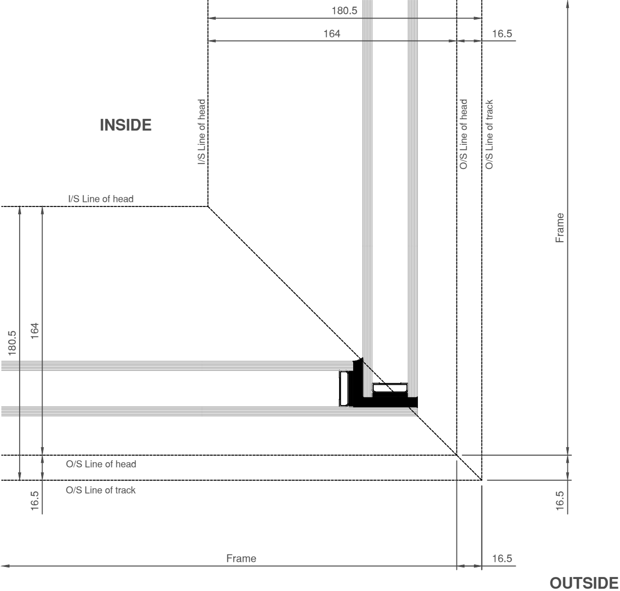
Glass-to-Glass HORIZONTAL SECTION
